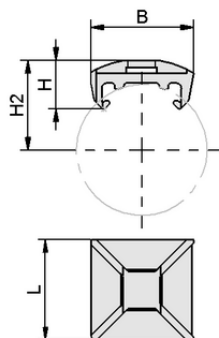
Design data HTR-D30-I FL PXT
