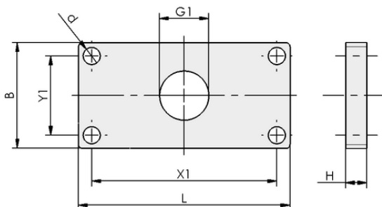
Design data VRS-PL-80x40 G1/2-IG MO-PROF
