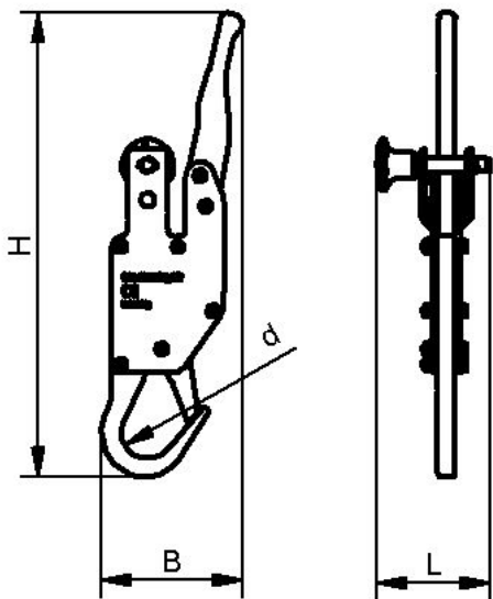
Design data EH-MON-28-d15x10 NEO30
