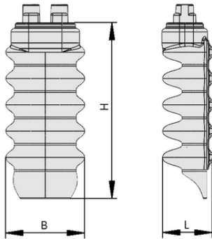
Design data FINGER-SPARE-UNIT 3CA IND
