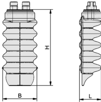
Design data FINGER-SPARE-UNIT 3C HYG
