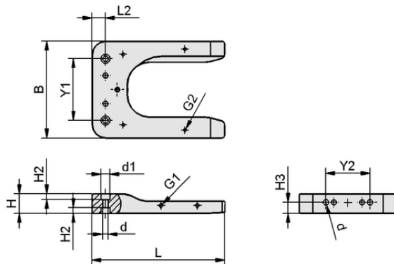
Design data STATION 150x110x22 MATCH
