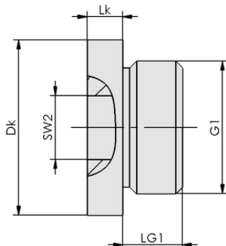
Design data VRS-SB G1/8-AG ISKT O-Ring
