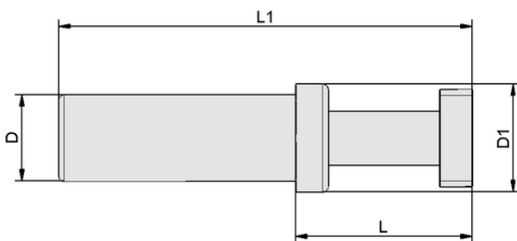
Design data VRS-STECH 8x18.5
