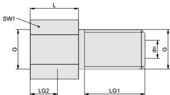
Design data VRL-S G1/8x15 MS-V
