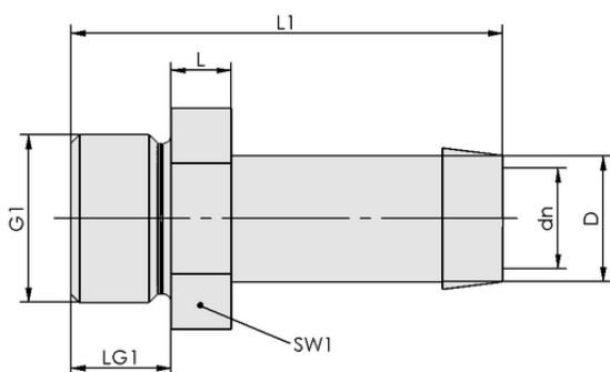
Design data ST G3/4-AG 13 MS-V
