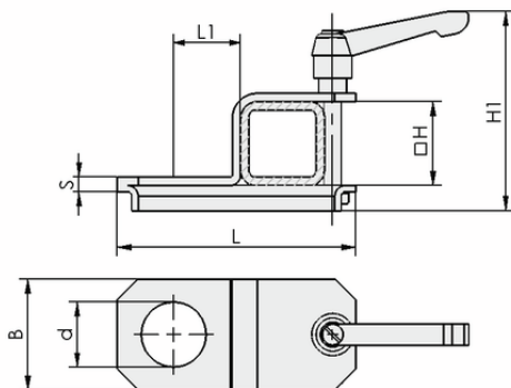
Design data HTR-STS 60x60 D30 WI
