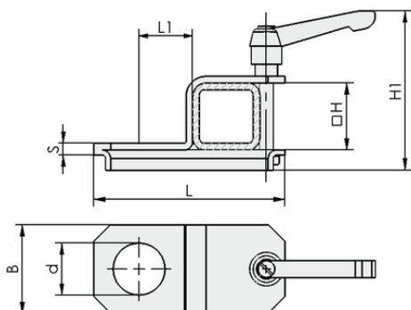
Design data HTR-STS 50x50 D30 WI
