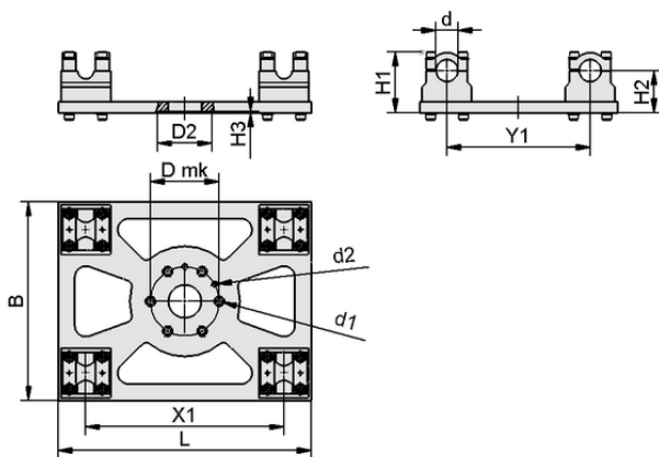
Design data SXT-RF-CL-D-160-40
