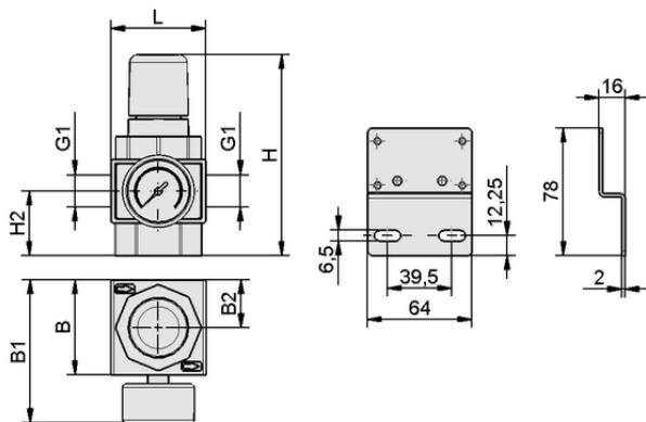
Design data DM 0.5...10 G1/2-IG
