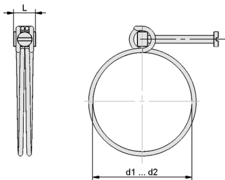
Design data SSD 85-90 ST-VZ
