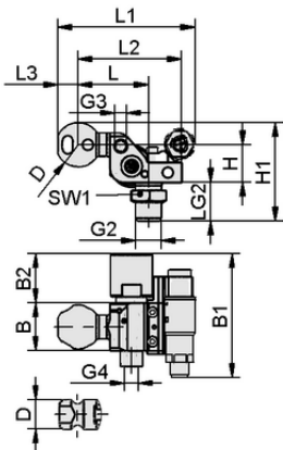
Design data HT-SG A3 I 10 31 NPT3/8-AG AB VS
