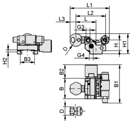
Design data HT-SG A2 I 10 46 RA AB VS
