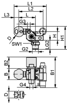
Design data HT-SG A3 I 10 31 NPT3/8-AG AB
