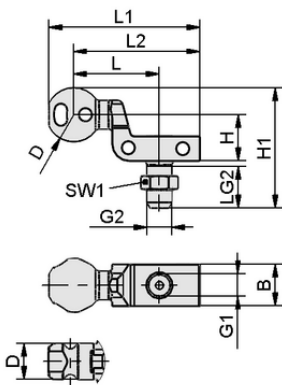
Design data HT-SG A3 22 NPT1/4-AG
