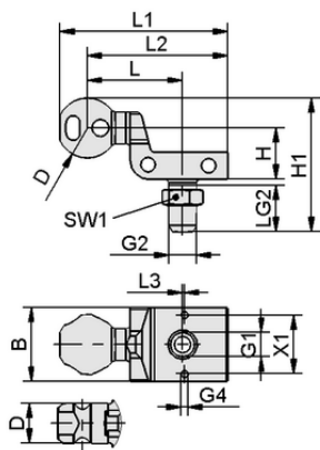
Design data HT-SG A2 E 35 NPT3/8-AG
