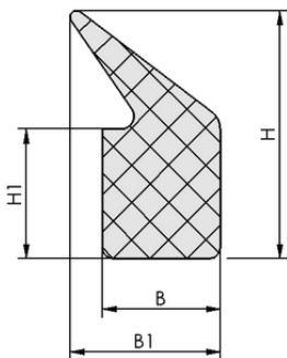
Design data DI-PROF 11x23 MOS CR-20 DL
