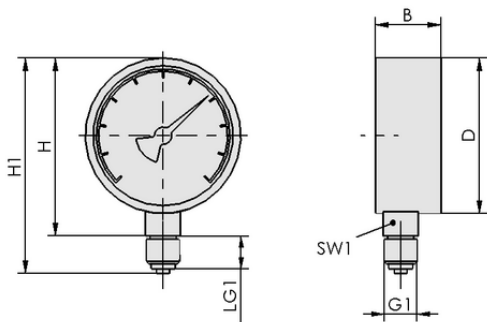
Design data VAM 40 V U BAR
