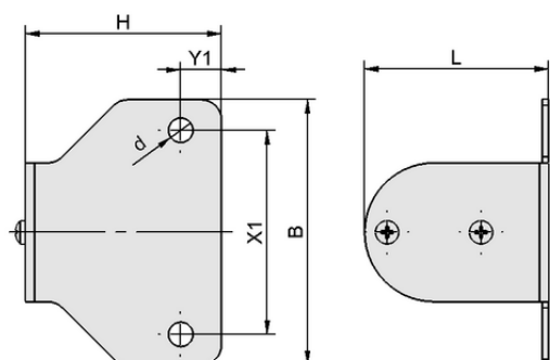
Design data HTR-FIL 2S WI VFT3/4
