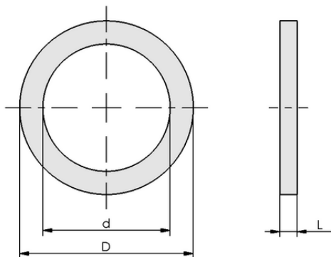
Design data DR 37-33x3 NBR
