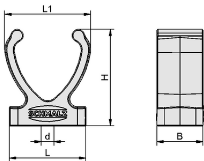
Design data HTR-VSi Clip
