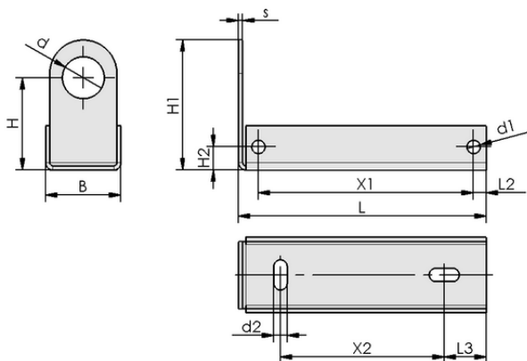
Design data BEF-WIN 21x22x39 1.5 VSi-M8
