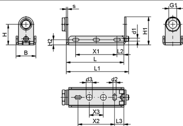
Design data BEF-WIN 21x22x61.5 1.5 VSi-D-M12
