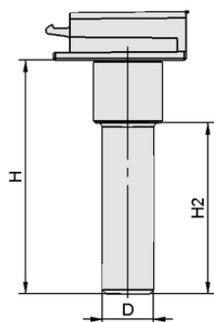
Design data ADAP-VS 6-1.3x16
