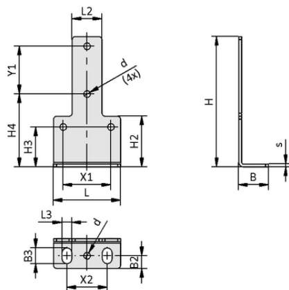
Design data BEF-WIN 45x20x87.35 LQE
