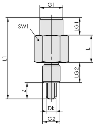
Design data TVN G1/4-AG 9 N009
