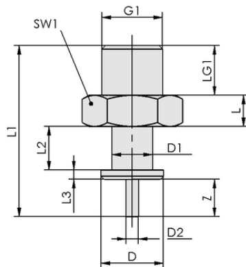
Design data TVN G1/4-AG 8.4 N041
