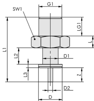
Design data TVN G1/8-AG 6.5 N008
