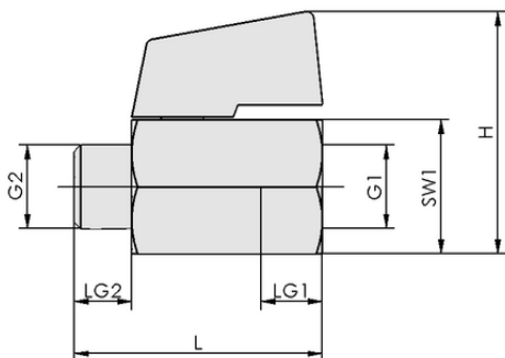
Design data KVZ 8 2/2
