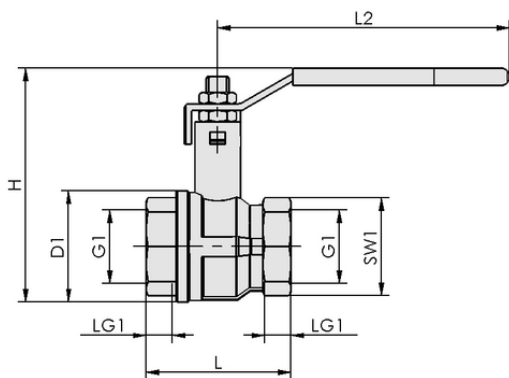
Design data KVZ 20 2/2
