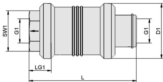
Design data HSV 12 3/2 G1/2-IG
