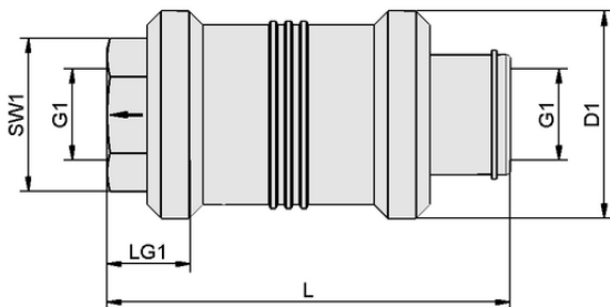
Design data HSV 7 3/2 G1/4-IG
