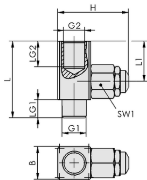
Design data DBV-M G1/4-AG MS
