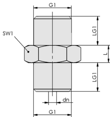
Design data SW 70 G1/4-AG
