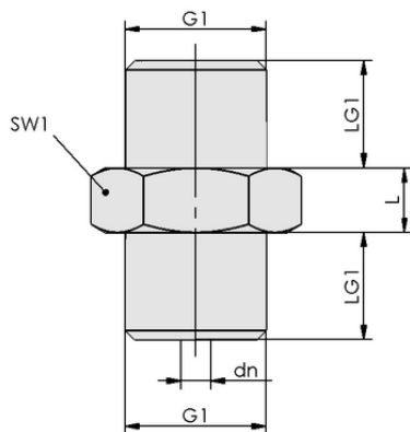
Design data SW 40 G1/8-AG
