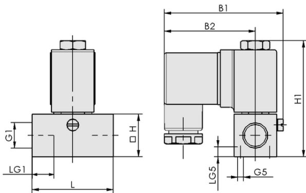
Design data EMV 3 230V-AC 2/2 NC
