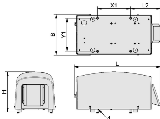
Design data SBB-EVE-24V-DC-ST-VZ-LUE
