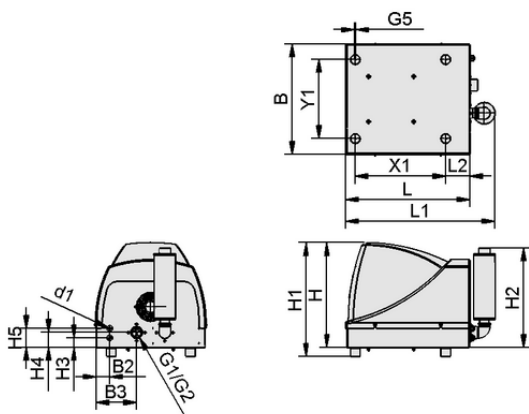
Design data SBB-230V-AC-ST/ABS-LUE SB
