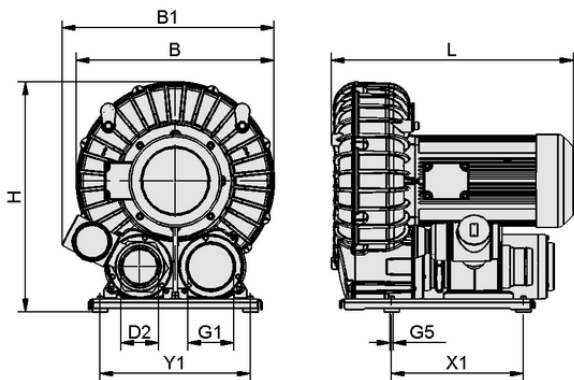
Design data SB 915 260 9 IE3-TYP2
