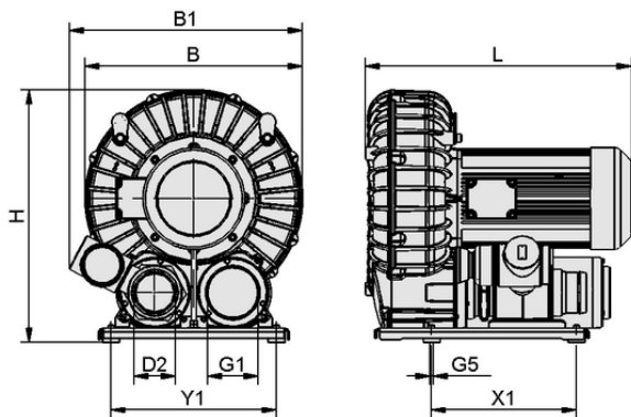
Design data SB 765 280 7.5 IE3-TYP3
