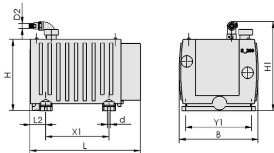
Design data EVE-WR 25 AC3
