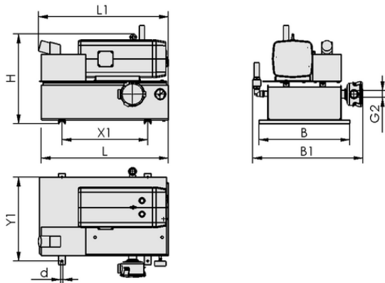
Design data VZ-OG 63 AC3 100 MS
