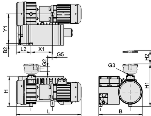
Design data EVE-OG 100 AC3 F IE3
