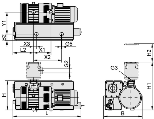
Design data EVE-OG 255 AC3 F
