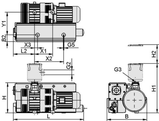
Design data EVE-OG 165 AC3 F
