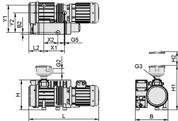
Design data EVE-OG 16 AC3
